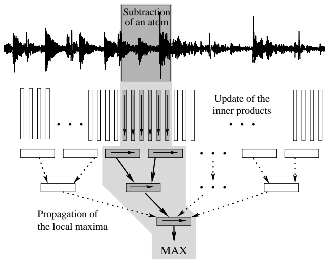
Fig. 1. Update of the inner products and maximum within a block: only the parts concerned with the subtraction of the previous atom (shaded parts) are updated.
